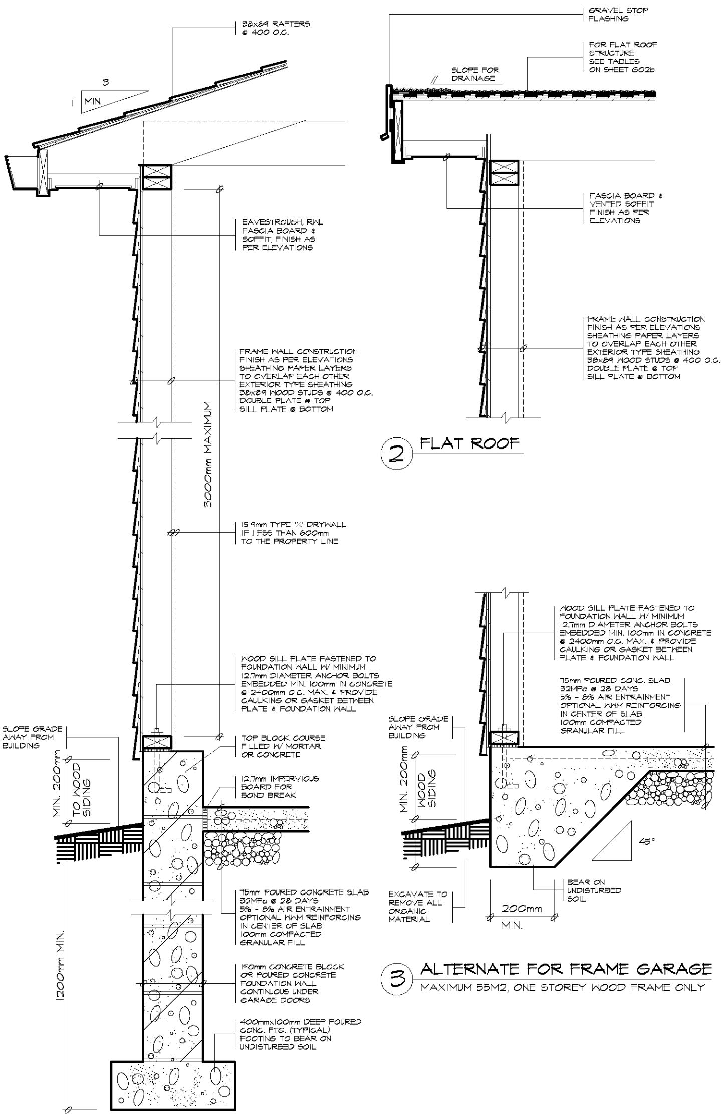
1 WALL SECTION
